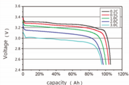
Discharge rate curves
