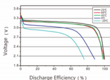
Temperature Characteristics
